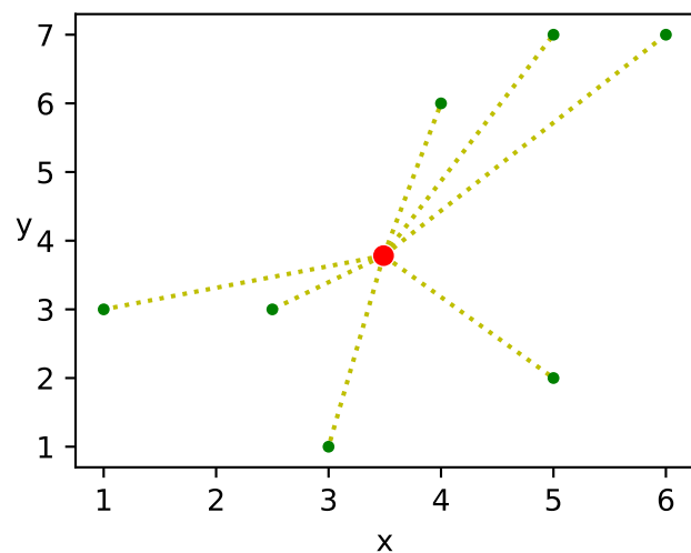
Geometric Median
